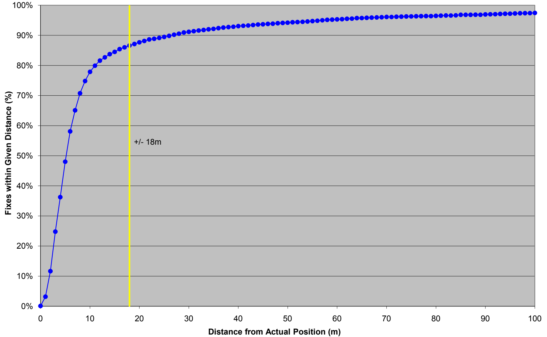
Graph of cumulative horizontal GPS fix accuracy (m) showing ~87% of all positions are within 18m of a known location.
