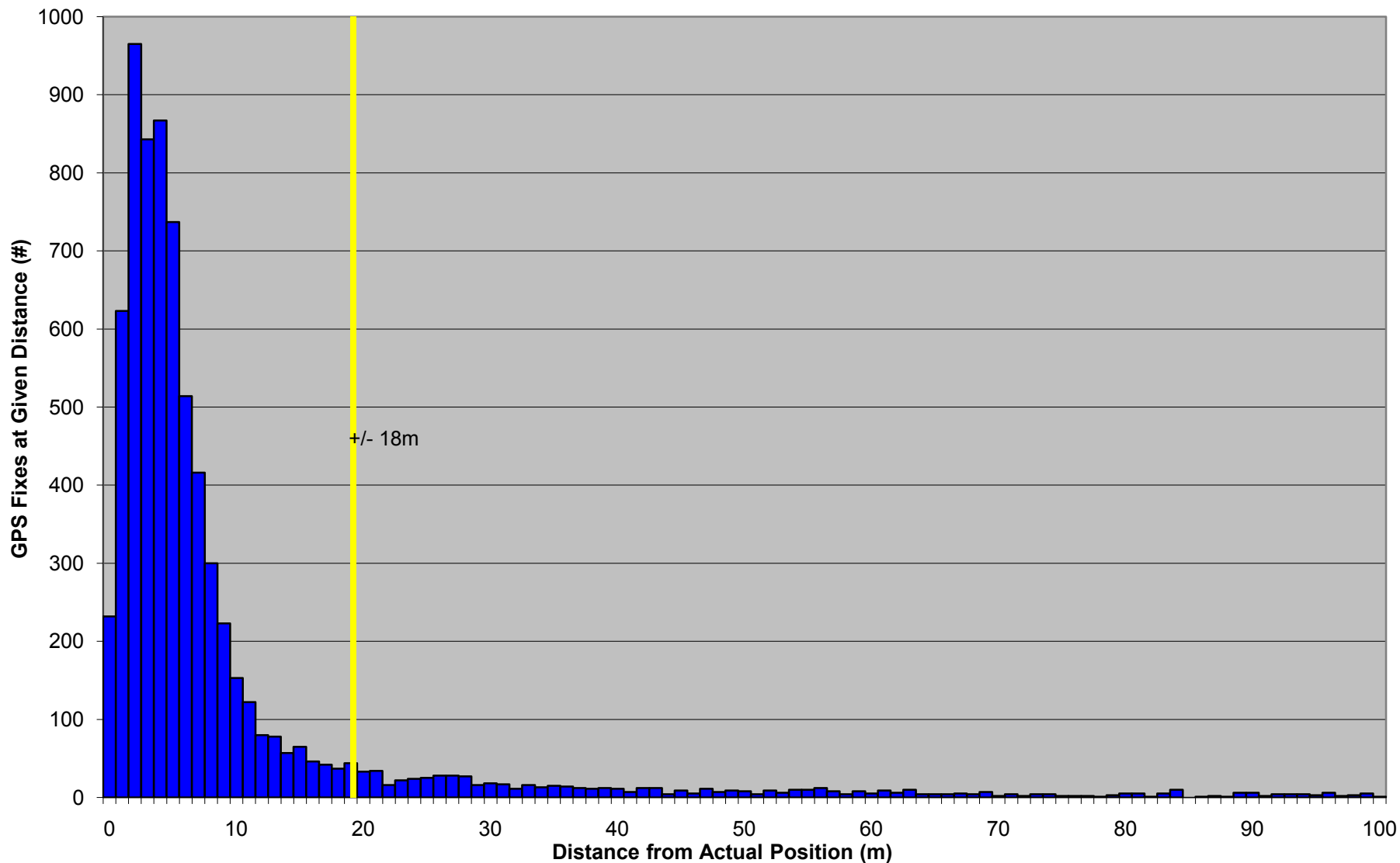
Histogram showing the frequency distribution of GPS fixes based on horizontal accuracy (m) from a known location.
